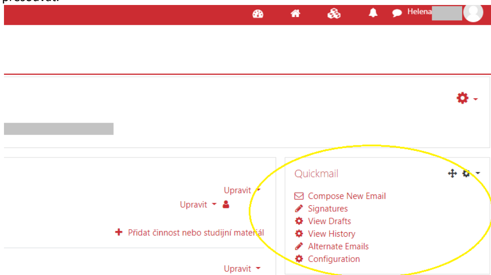
Obr. 5: Quickmail
